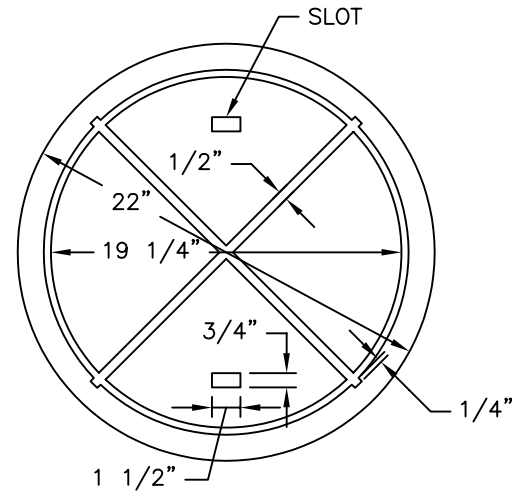
PLAN - COVER BOTTOM
